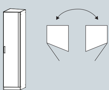
OX5U hinged door robe, angled w 47, h 212, d 56
